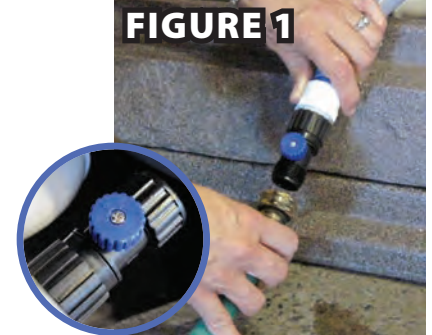
GATE VALVE/CLIP
